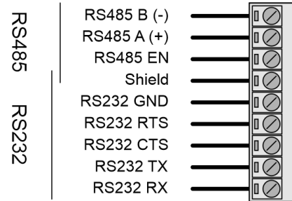
PLX51-DNPM and PLX51-DNPS Auxiliary Communication Connector:
