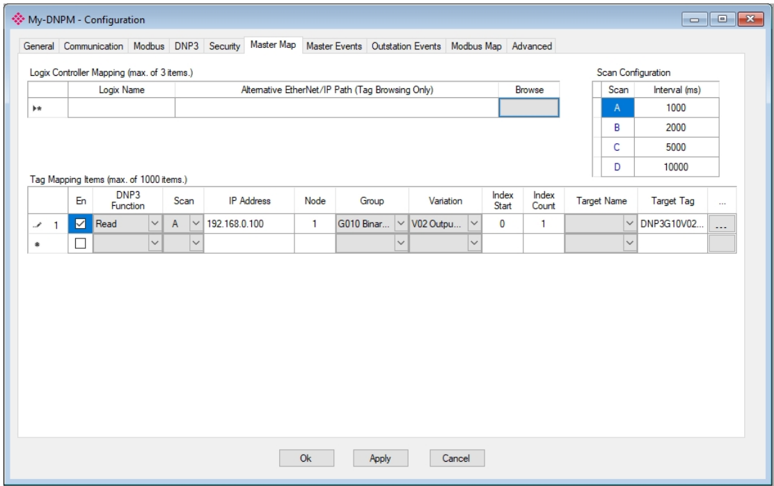
Figure 3.28 – Master configuration with CIP USB Logix
