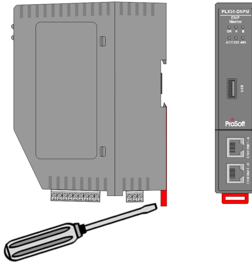
Figure 2.4 - DIN rail mounting
