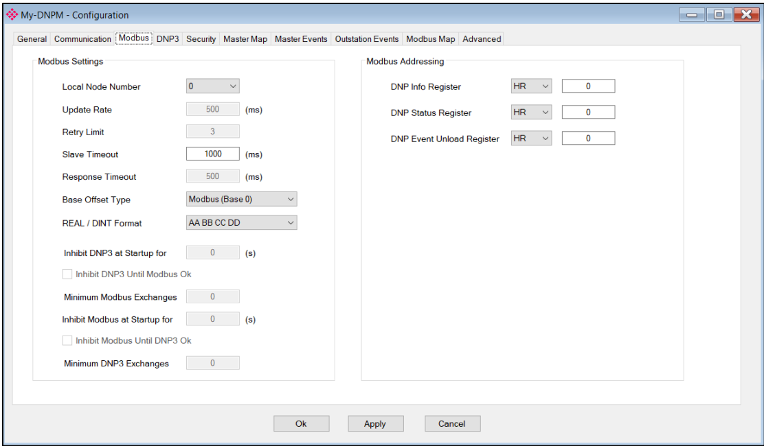
Figure 3.16. - Modbus Configuration
