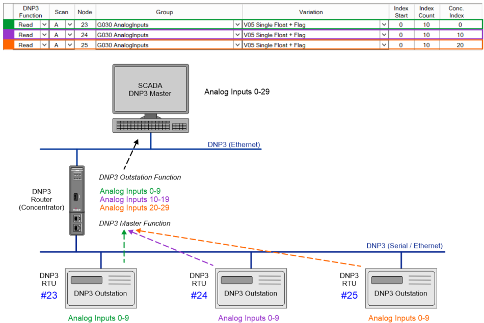
Figure 3.38 – Concentrator Example
