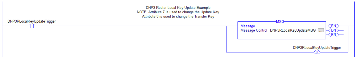
Figure 8.2 - Message Instruction
