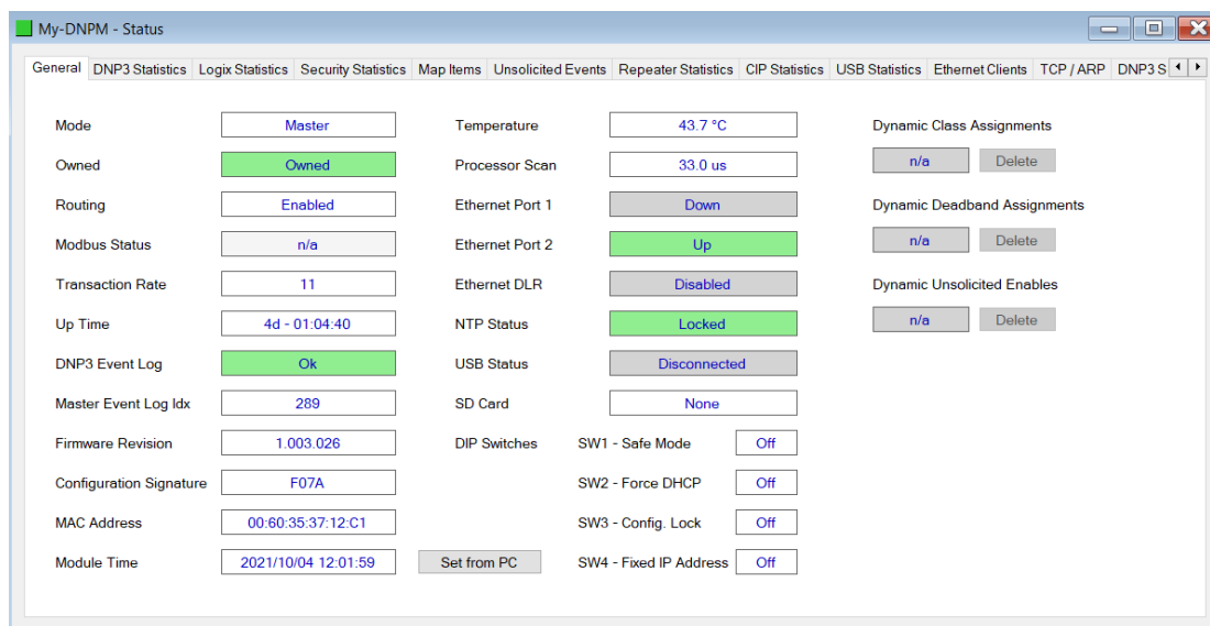
Figure 9.4 – General Status
