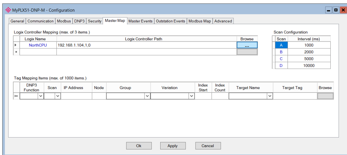
Figure 3.23 - Master configuration
