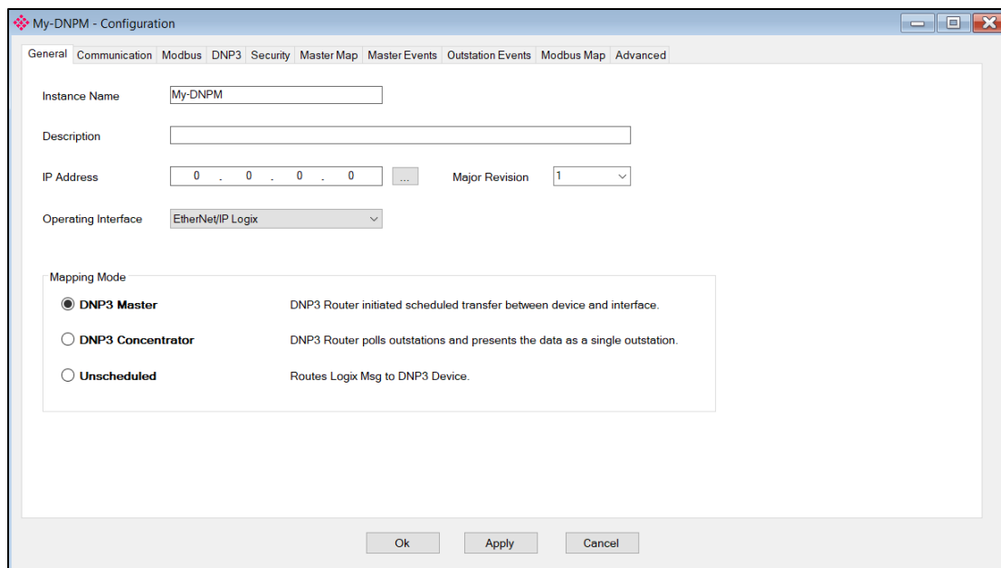
Figure 3.13. – PLX51-DNPM configuration
