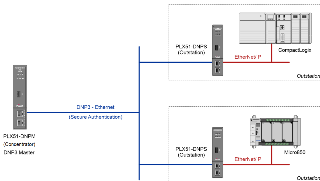
Figure 1.1. – Typical Setup
