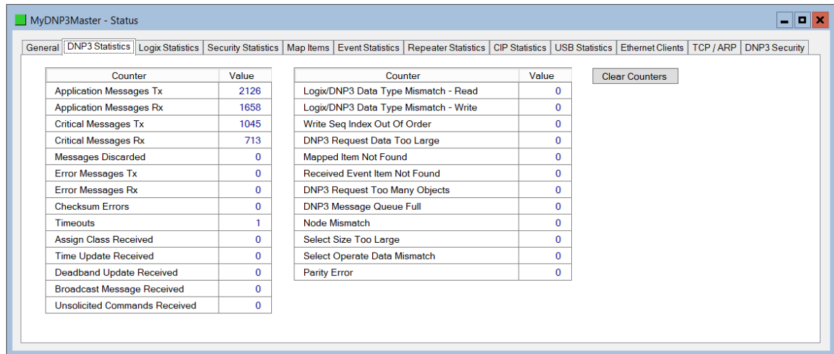
Figure 9.5. – DNP3 Statistics
