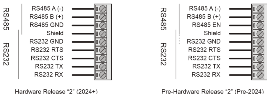
Figure 2.6 - RS232/RS485 connector
