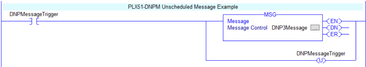
Figure 5.2 - Message Instruction
