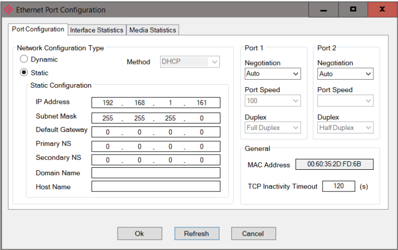
Figure 3.9. - Port Configuration
