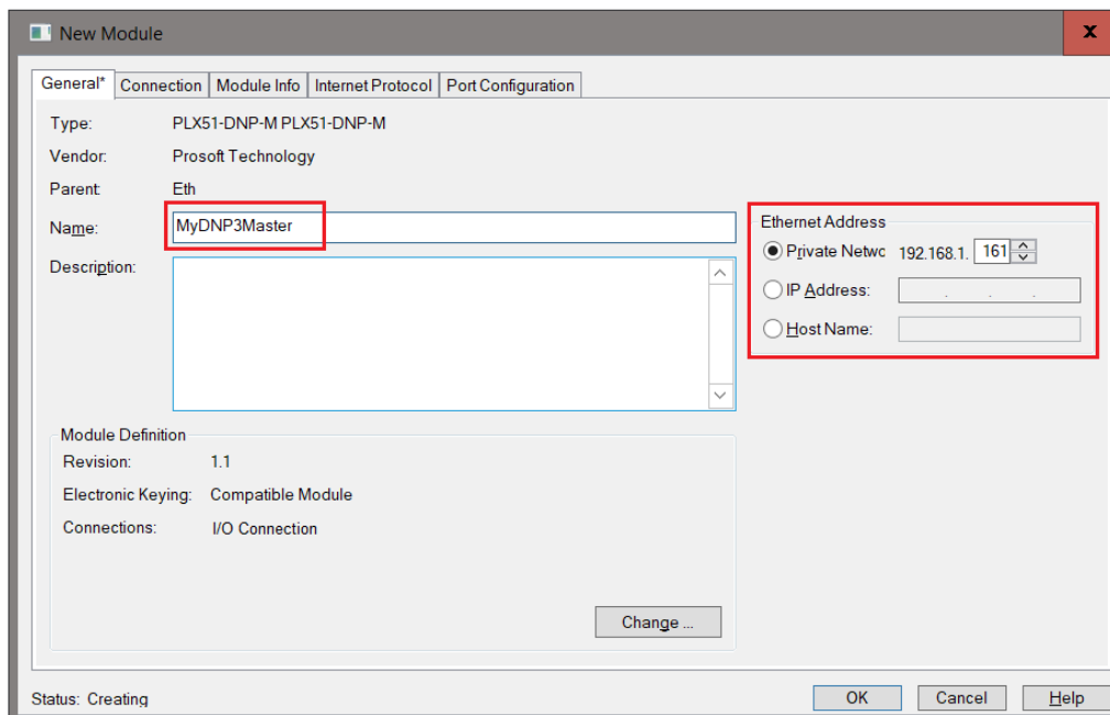
Figure 3.53 – Module instantiation
