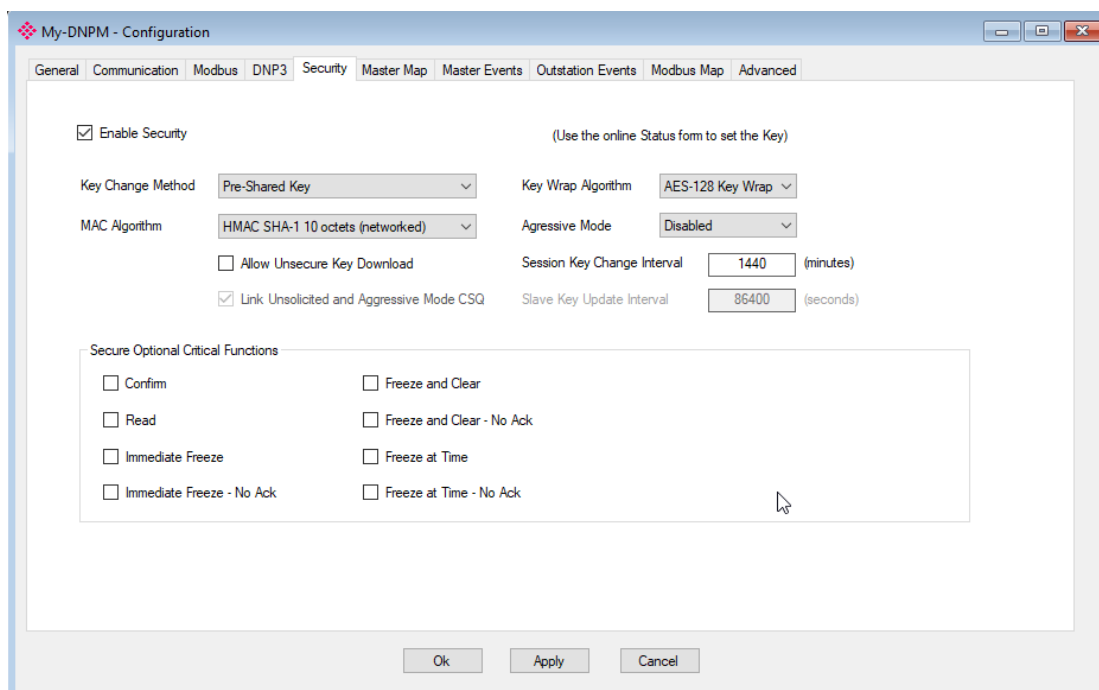
Figure 3.18 - Security configuration
