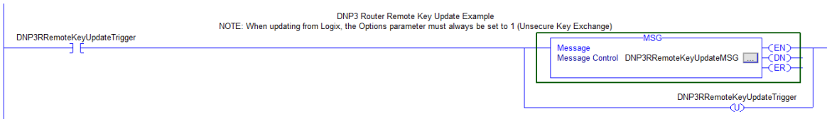
Figure 8.6 - Message Instruction
